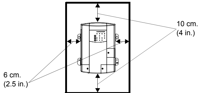
Figure 7 Ventilation Clearance
