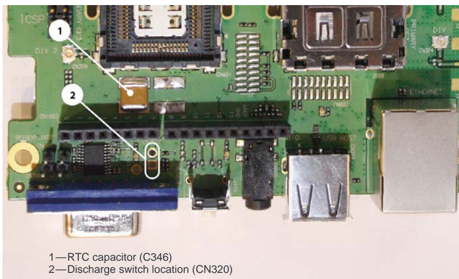
Figure 3-11: RTC Capacitor
