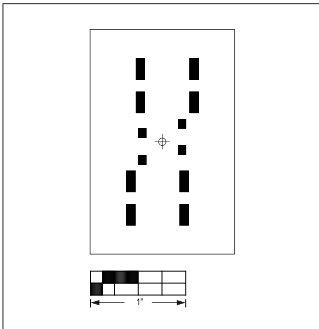
MAX86141OSBEK#—Bottom
