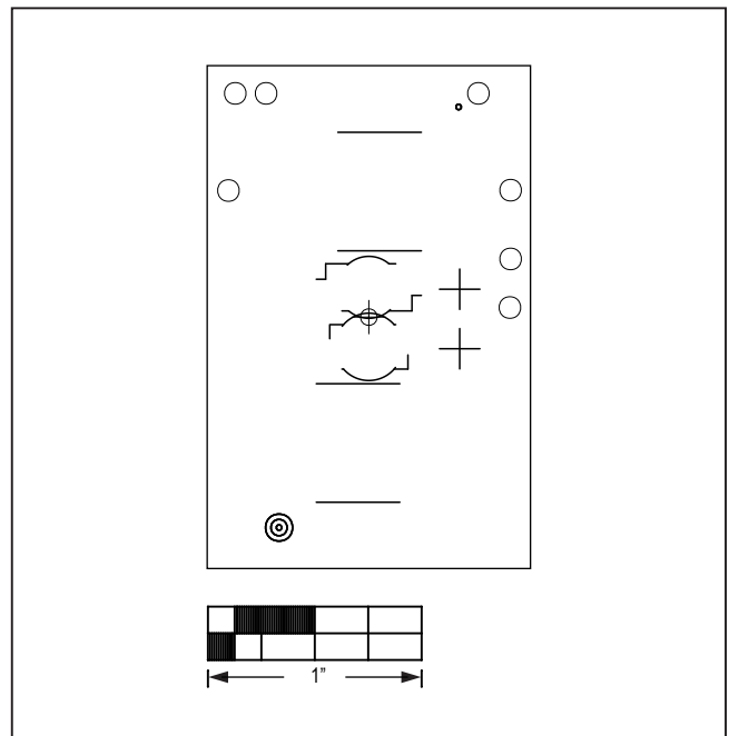
MAX86141OSBEK#—Bottom Silkscreen
