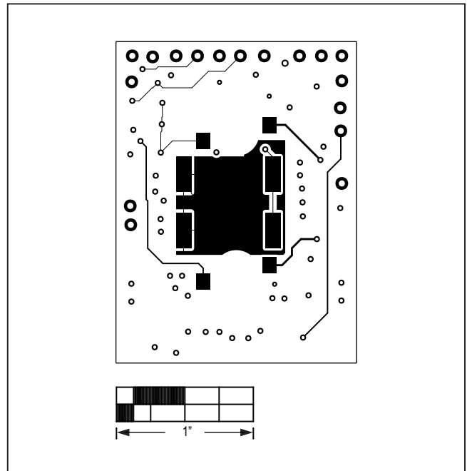
MAX86140SBEK#—Bottom
