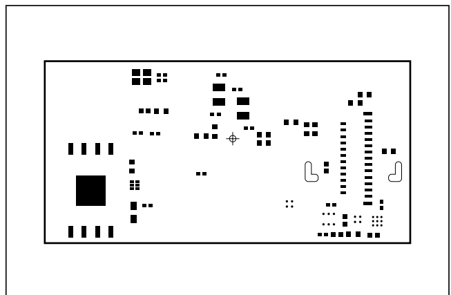
MAX32620UCBLEEK#—Bottom Paste
