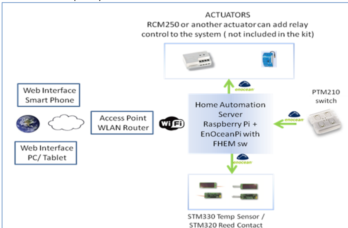
Figure 1: Home Automation Using Raspberry Pi & EnOcean Pi
