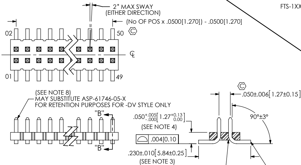
FIG 2 FTS-1XX-03-XX-DV SHOWN (DIFFERENT AS SHOWN, OTHERWISE SAME AS FIG 1)
