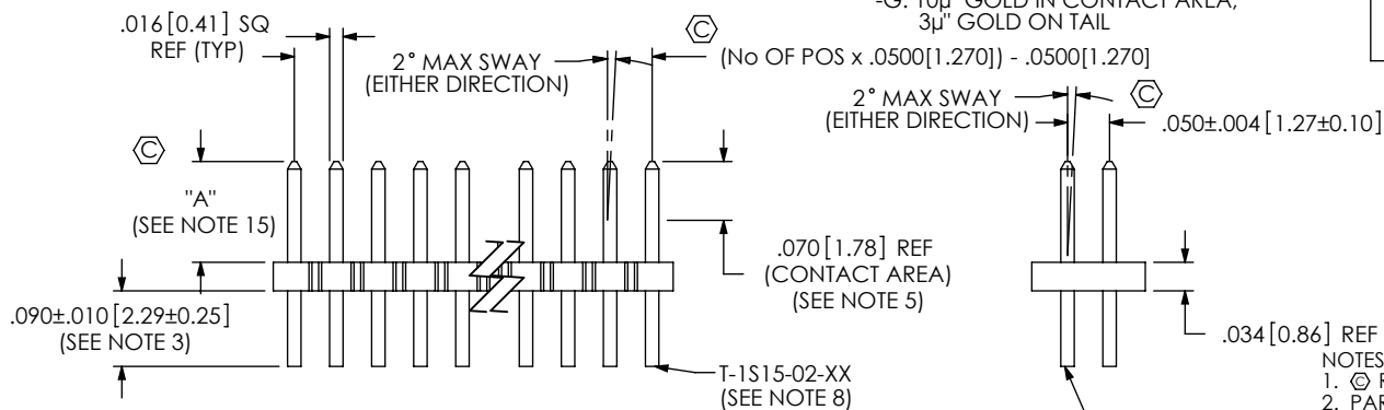
FIG 1 FTS-1XX-0T-XX-D SHOWN
