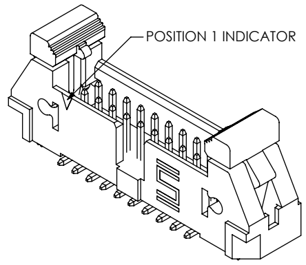
FIG 1 EJH-110-01-X-D-SM-LC SHOWN NOTES: ⊕ REPRESENTS A CRITICAL DIMENSION. COPLANARITY TO BE: .004 MAX FOR POSITIONS -05 THRU -10 .006 MAX FOR POSITIONS -15 THRU -25 BURR ALLOWANCE: .0015 MAX. MINIMUM PUSHOUT FORCE: 1 LB MIN. MAXIMUM ALLOWABLE BOW: .002 INCH/INCH AFTER ASSEMBLY. PARTS TO BE TUBED WITH EJECTOR ARMS IN THE UP POSITION AS SHOWN. REPRESS TO DIMENSION SHOWN. NOTE DELETED. MEASURE FROM THE TIPS OF THE TERMINALS. DUE TO THE HIGH AMOUNT OF INSERTION FORCE NEEDED, THE -LC OPTION IS NOT COMPATIBLE WITH AUTO PLACEMENT. SAMTEC RECOMMENDS MANUAL PLACEMENT FOR ALL ASSEMBLIES WITH THE -LC OPTION.
