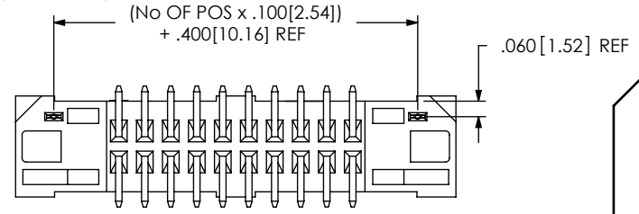
FIG 1 EJH-110-01-X-D-SM-LC SHOWN NOTES: ⊕ REPRESENTS A CRITICAL DIMENSION. COPLANARITY TO BE: .004 MAX FOR POSITIONS -05 THRU -10 .006 MAX FOR POSITIONS -15 THRU -25 BURR ALLOWANCE: .0015 MAX. MINIMUM PUSHOUT FORCE: 1 LB MIN. MAXIMUM ALLOWABLE BOW: .002 INCH/INCH AFTER ASSEMBLY. PARTS TO BE TUBED WITH EJECTOR ARMS IN THE UP POSITION AS SHOWN. REPRESS TO DIMENSION SHOWN. NOTE DELETED. MEASURE FROM THE TIPS OF THE TERMINALS. DUE TO THE HIGH AMOUNT OF INSERTION FORCE NEEDED, THE -LC OPTION IS NOT COMPATIBLE WITH AUTO PLACEMENT. SAMTEC RECOMMENDS MANUAL PLACEMENT FOR ALL ASSEMBLIES WITH THE -LC OPTION.
