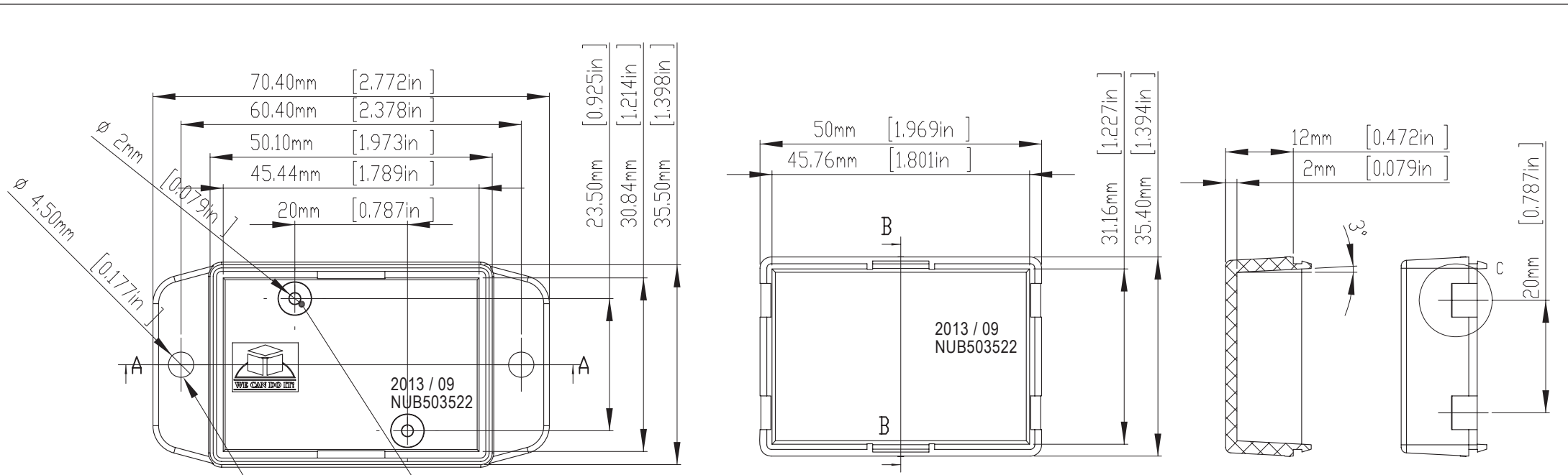
SECTION B-B SCALE 1.5 : 1
