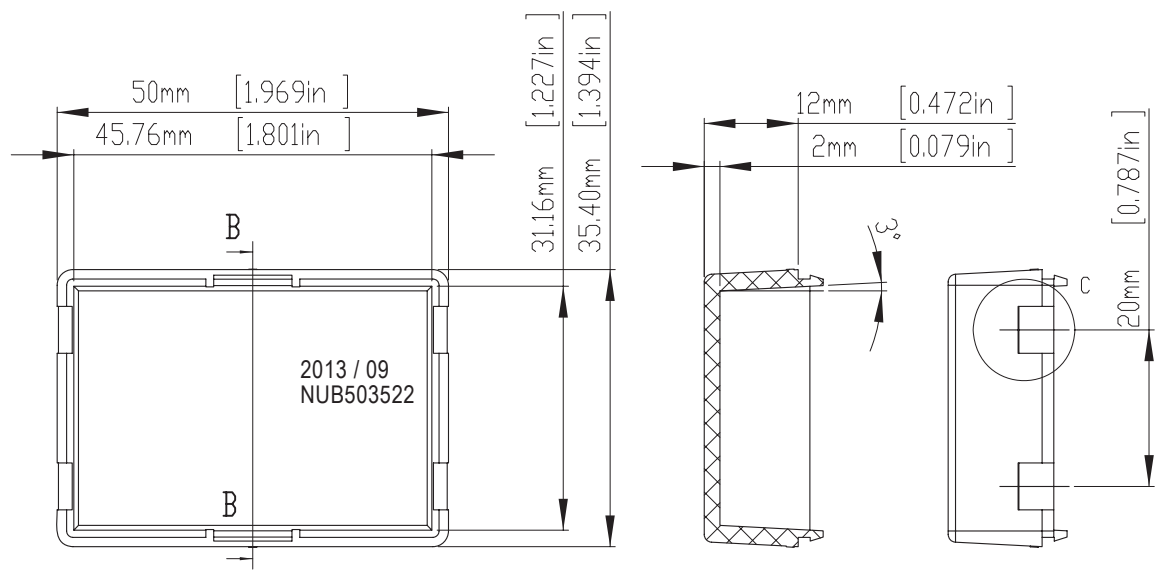
SECTION B-B SCALE 1.5 : 1
