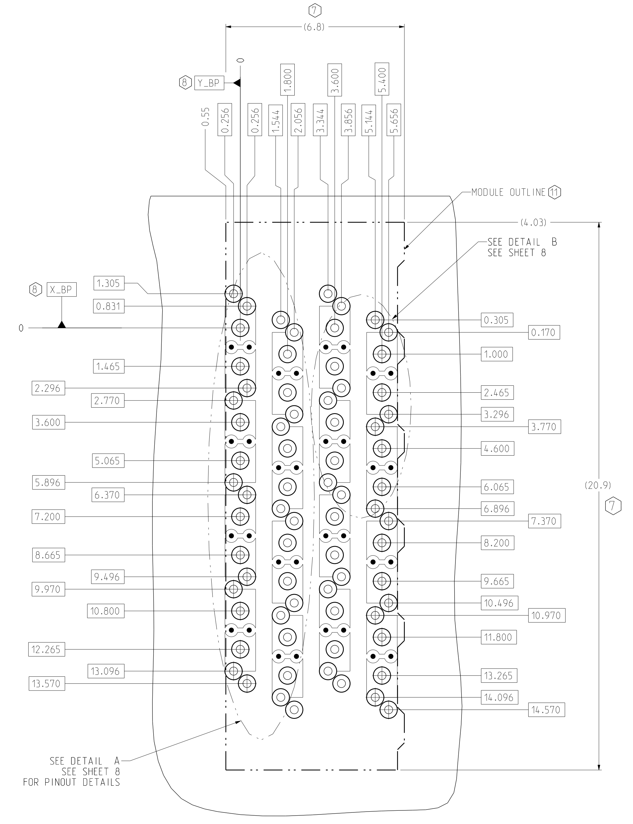
BP HOLE PATTERN COMPONENT SIDE SCALE 12/1
