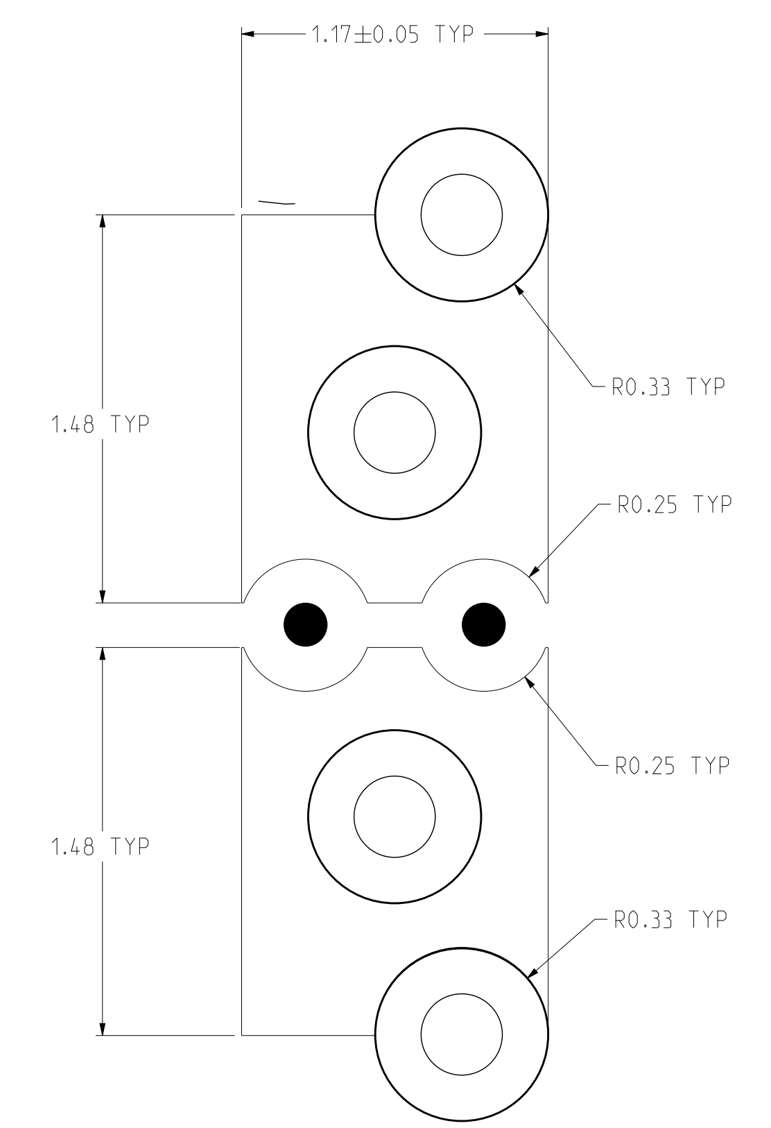
DETAIL C ANTI PAD DETAILS GROUND AND SHADOW VIAS CAN BE CONNECTED AS ONE CONTINUOUS SURFACE PAD SCALE 50/1
