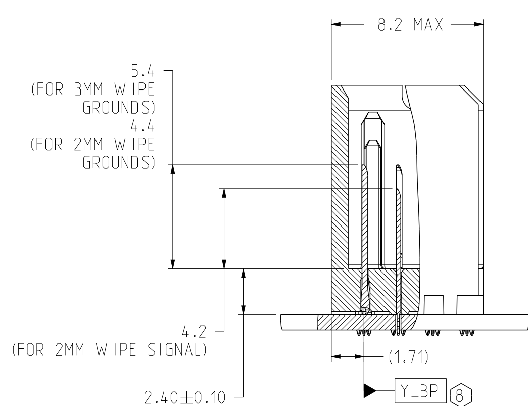
SECTION Z-Z
