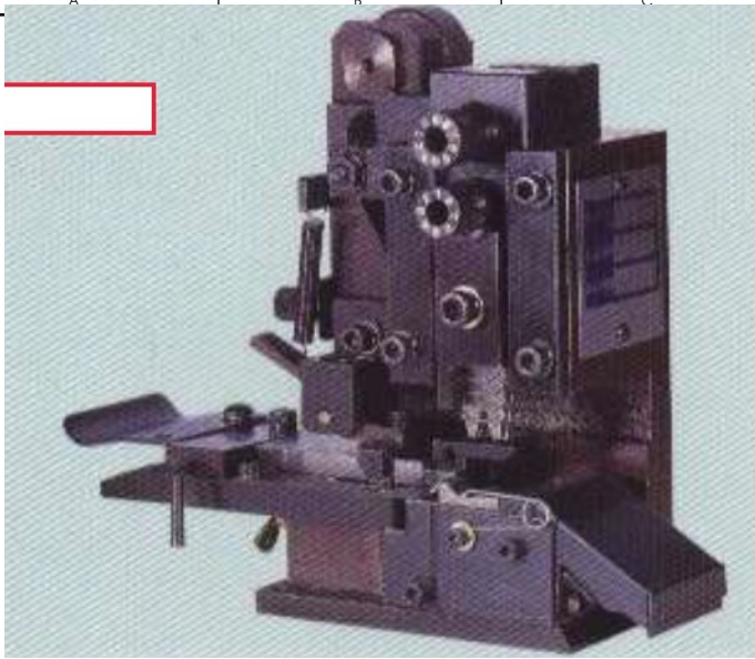
FLH-CT-S-02 APPLICATOR
