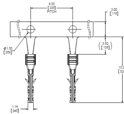
SOCKET CONTACT FLH-SC136-T01
