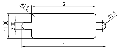
RECOMMENDED PANEL CUT-OUT Tolerance: ±0.05mm
