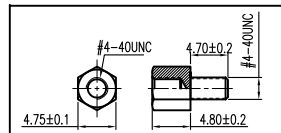
4.8*9.5 SCREW
