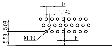
RECOMMENDED P.C.B LAYOUT Tolerance: ±0.05mm
