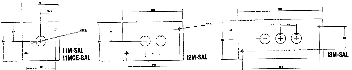
Enclosure dimensions over outside of cover Enclosure depth 67mm
