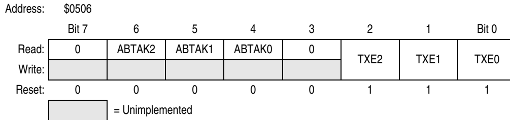
Figure 12-22. Transmitter Flag Register (CTFLG)
