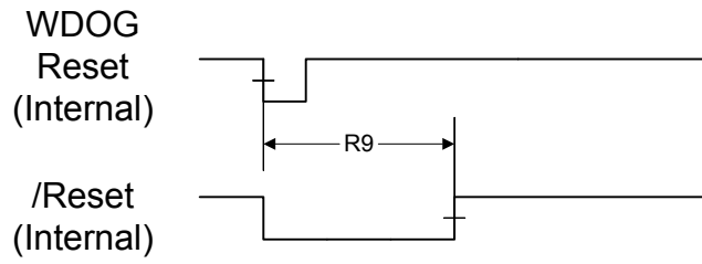
Figure 22-15. Watchdog Reset Timing
