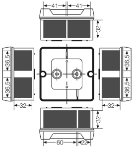
Dimension drawing
