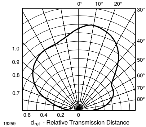
Fig. 13 - Vertical Directivity
