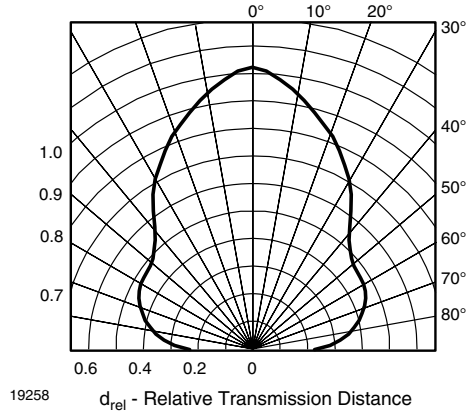
Fig. 12 - Horizontal Directivity
