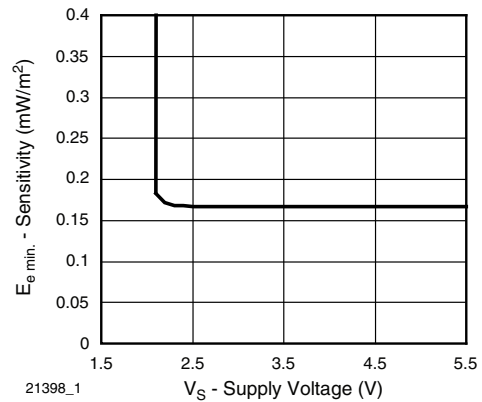
Fig. 14 - Sensitivity vs. Supply Voltage
