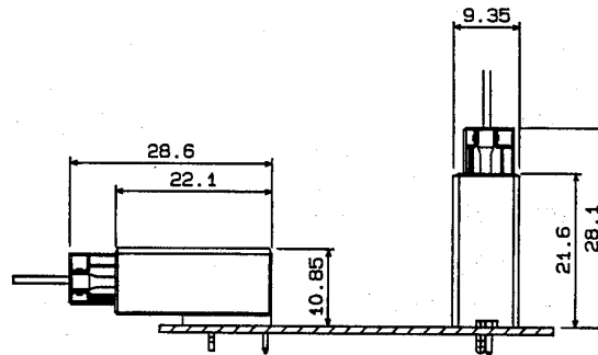
Horizontal/Vertical Type
