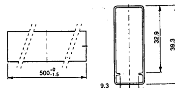
Tube Package Dimensions (Ref.)
