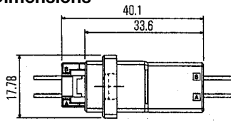
Panel/Free-Hanging Type
