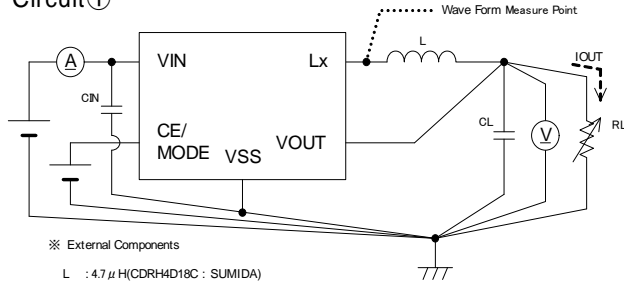
Circuit①
