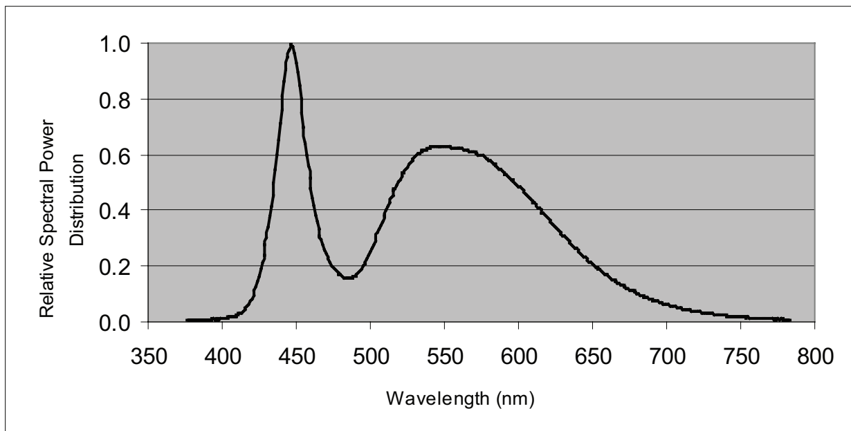
Figure 5. White Color Spectrum of Typical CCT Part, Integrated Measurement.
