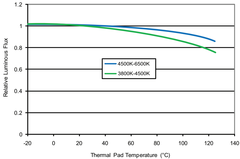
Figure 6. Relative Light Output vs. Thermal Pad Temperature.
