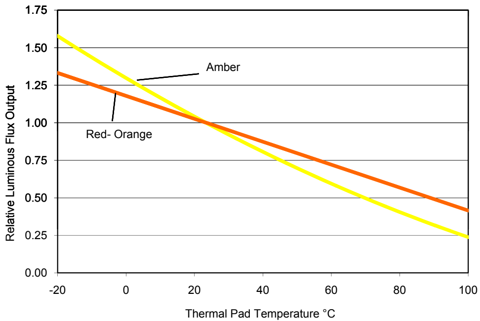
Figure 7. Relative Light Output vs. Junction Temperature for Red-Orange and Amber.
