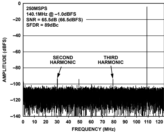
Figure 6. Single-Tone FFT with f_{IN} = 140.1 MHz
