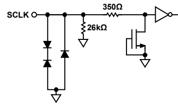
Figure 22. Equivalent SCLK Input Circuit
