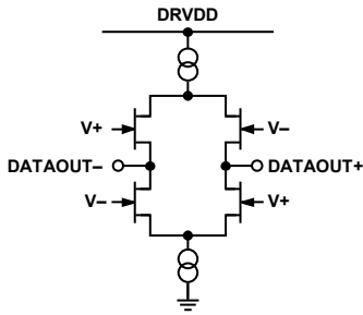
Figure 20. Equivalent LVDS Output Circuit
