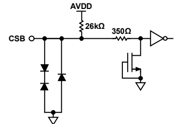
Figure 23. Equivalent CSB Input Circuit
