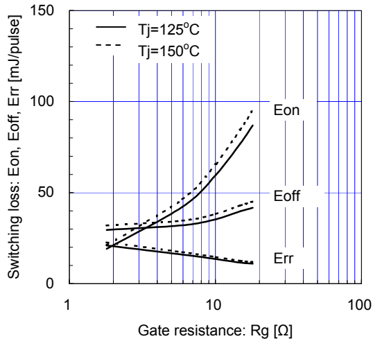
Switching loss vs. Gate resistance (typ.) V_{cc}=600V, I_c=300A, V_{GE}=\pm 15V, T_j=125^\circ C
