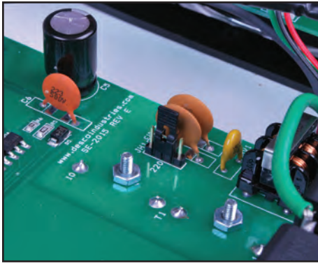
Figure 4. 220 volt jumper setting
