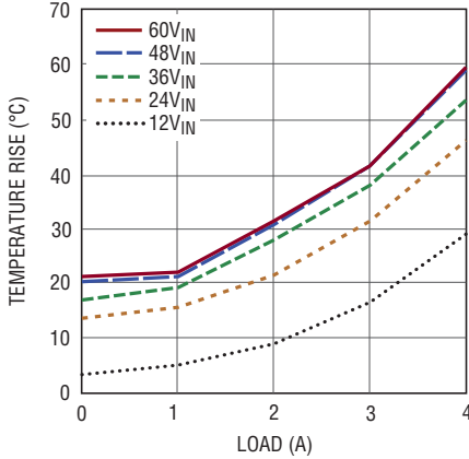
Temperature Rise vs Load, V_{OUT} = 8\text{V}
