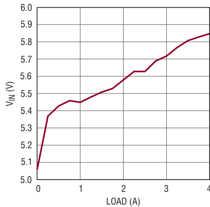
Minimum V_{IN} vs Load, V_{OUT} = 5V
