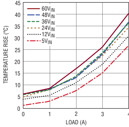
Temperature Rise vs Load, V_{OUT} = 3.3\text{V}
