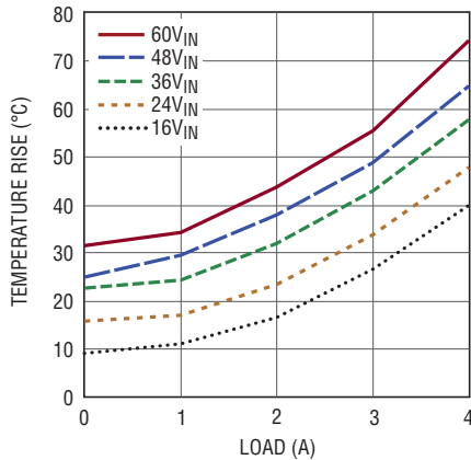
Temperature Rise vs Load, V_{OUT} = 12\text{V}
