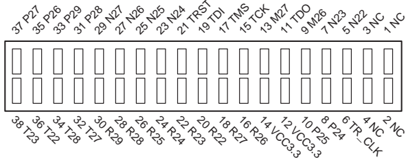
Figure 8. Debug Mictor Connector - J20
