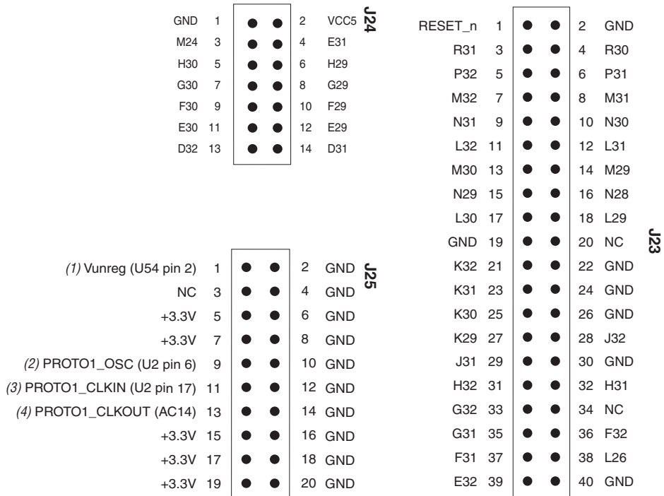
Figure 11. Expansion Prototype Connector Pin Information - J23, J24, J25
