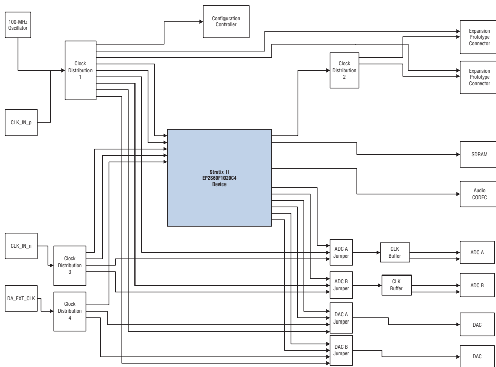
Figure 3. Clock Distribution
