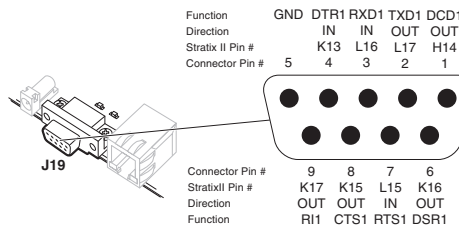
Figure 9. Serial Connector J29
