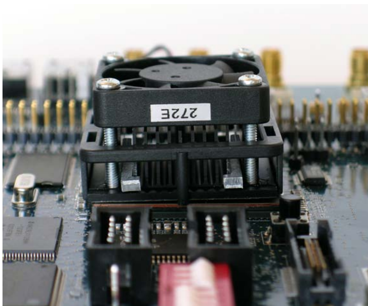
Figure 14. Tilt the Heat Sink
