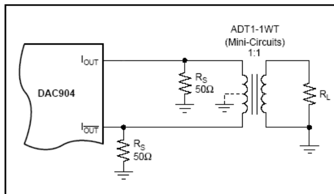
Figure 5. On-Board Circuitry after D/A Converter
