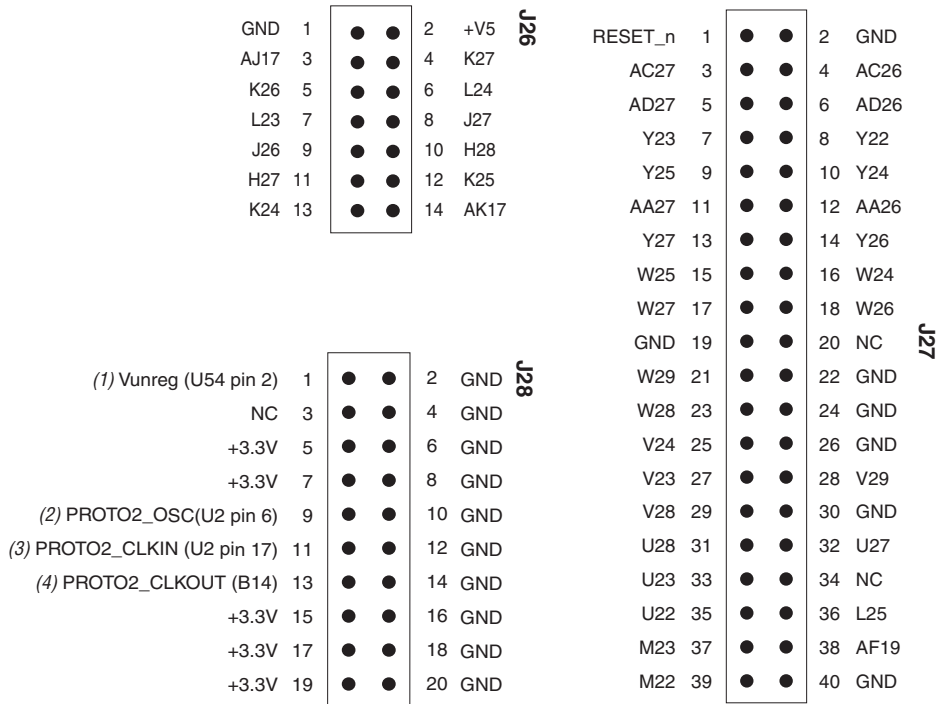
Figure 13. Expansion Prototype Connector -Pin Information for J26, J27, & J28
