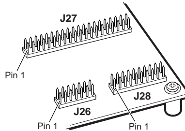
Figure 12. Expansion Prototype Connector - J26, J27, J28
