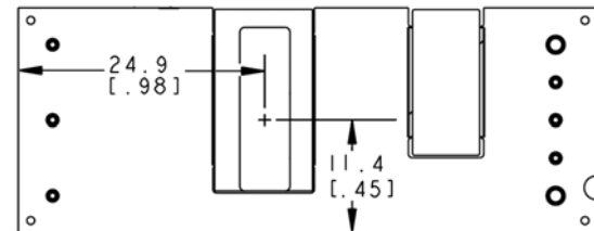
Figure 21. Pick and Place Location.
