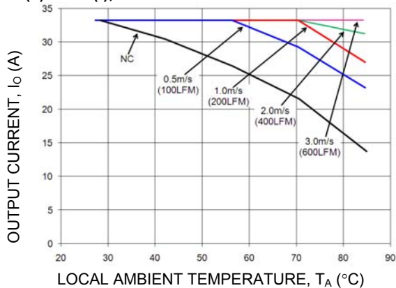
Figure 23. Output Current Derating for the Base plate QBDW033A0B-H with 1.0" heatsink in the Transverse Orientation; Airflow Direction from Vin(+) to Vin(-); Vin = 48V.
