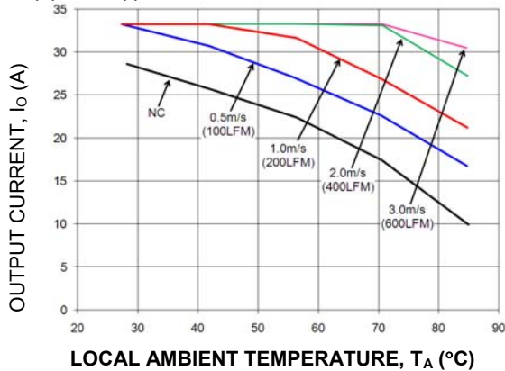
Figure 22. Output Current Derating for the Base plate QBDW033A0B-H with 0.5" heatsink in the Transverse Orientation; Airflow Direction from Vin(+) to Vin(-); Vin = 48V.
