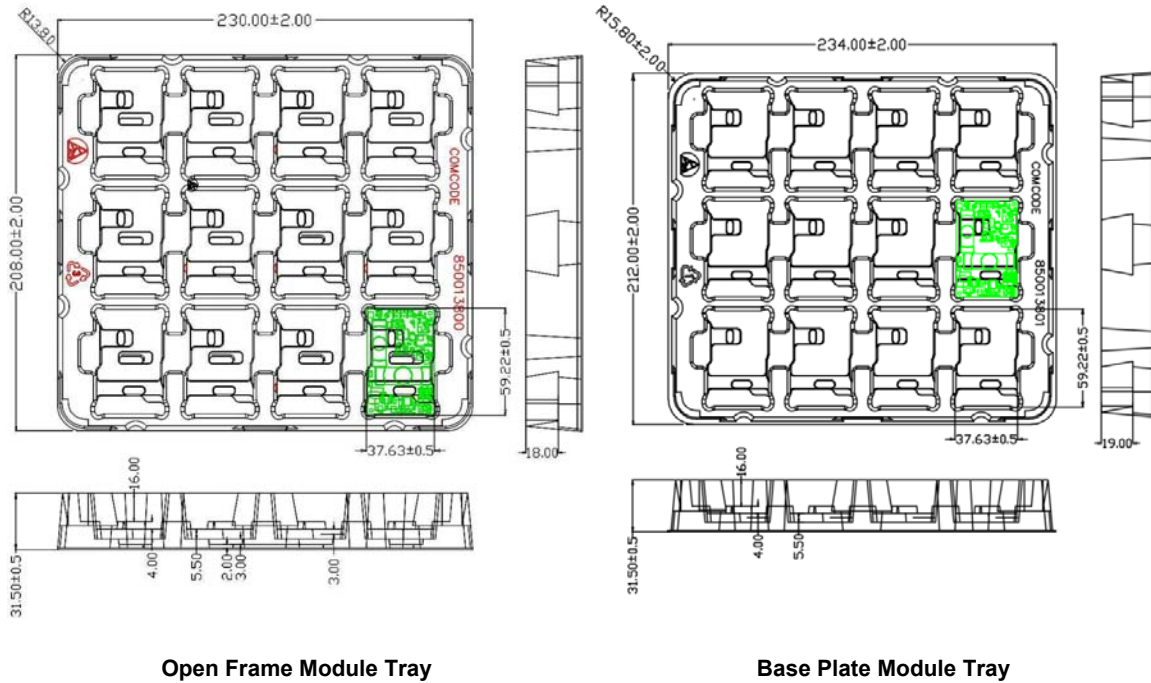
Figure 26. QBDW033 Packaging Tray
