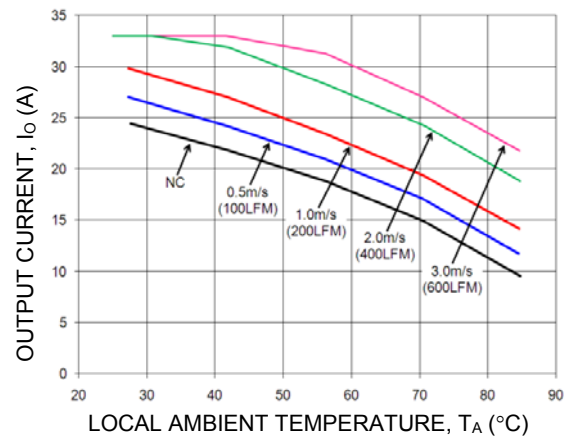
Figure 19. Output Current Derating for the Open Frame QBDW033A0B in the Transverse Orientation; Airflow Direction from Vin(+) to Vin(-); Vin = 48V.
