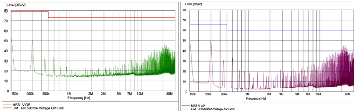
Figure 25. EMC Consideration
