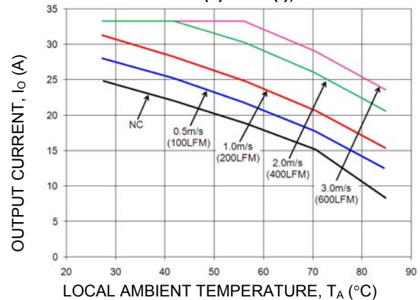
Figure 20. Output Current Derating for the Baseplate QBDW033A0B-H in the Transverse Orientation; Airflow Direction from Vin(+) to Vin(-); Vin = 48V.
