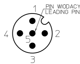
WIDOK OD STRONY DRUTOW VIEW FROM WIRES SIDE
