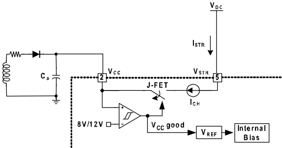
Figure 14. Startup Circuit
