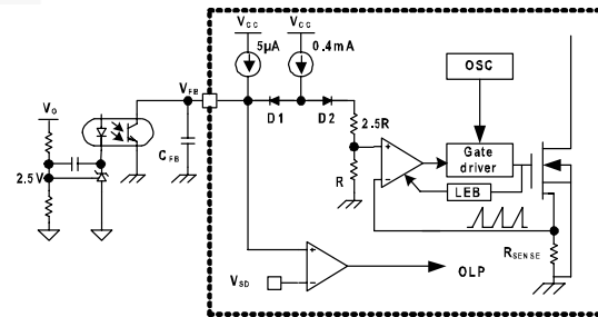
Figure 16. Pulse-Width-Modulation Circuit
