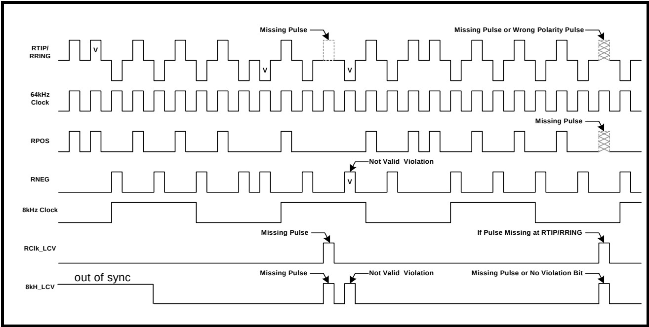
FIGURE 3. INPUT DATA 64 KHz + 8 KHz OPERATION (s1 = 0, s2 = 0, s3 = 0)
