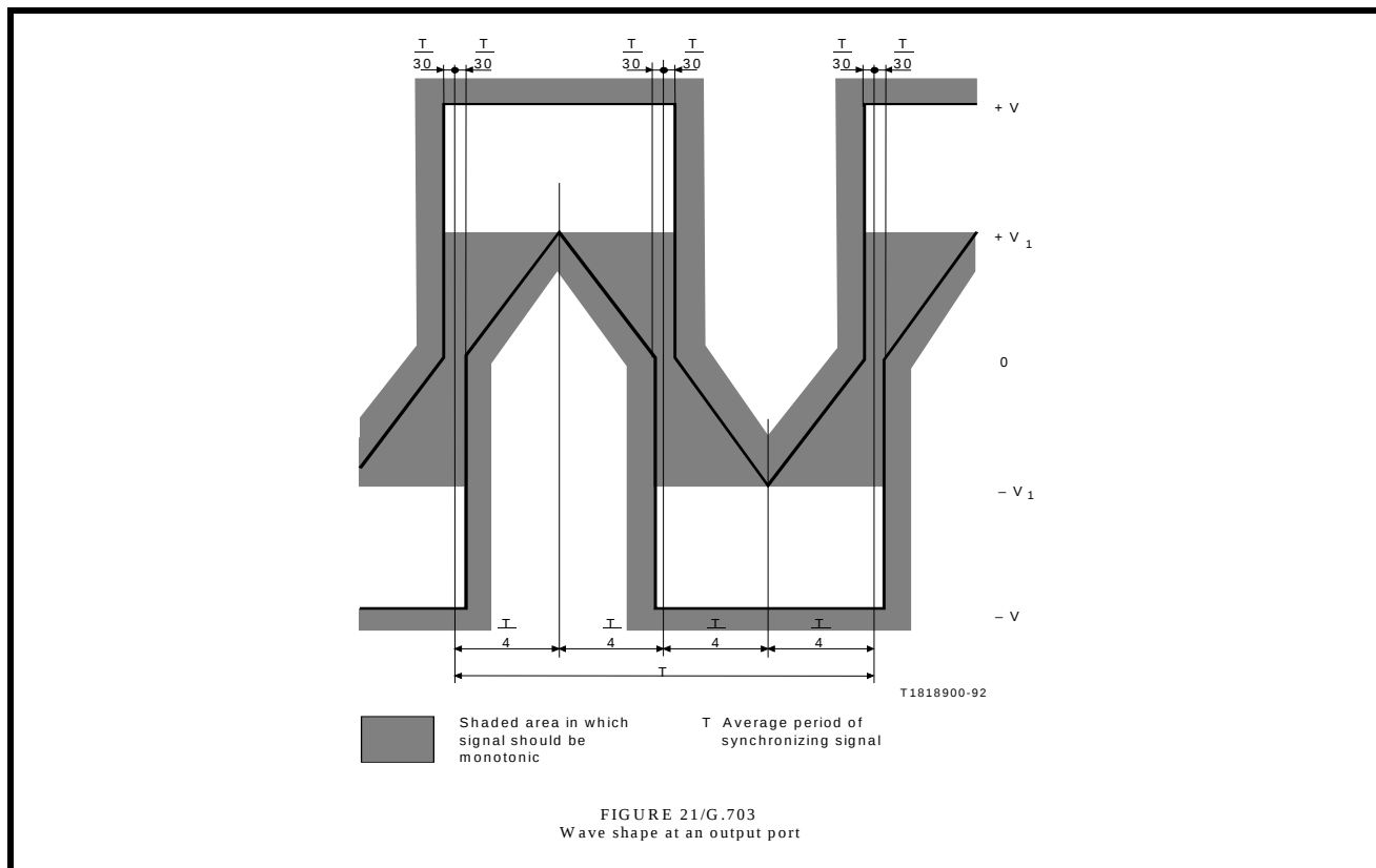
FIGURE 6. E1 CLOCK SIGNAL WAVE SHAPE - G.703
