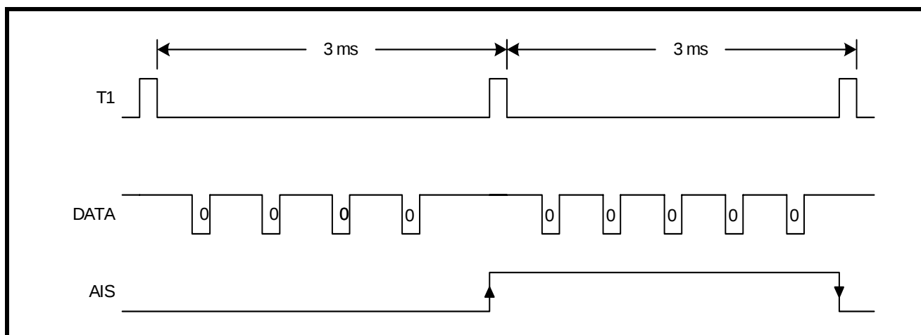
FIGURE 9. AIS DETECTION FOR T1 MODE
