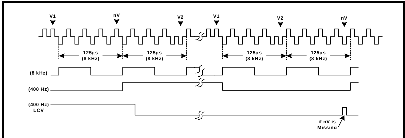
FIGURE 4. INPUT DATA 64 KHz + 8 KHz + 400 Hz OPERATION (s1 = 0, s2 = 0, s3 = 1)
