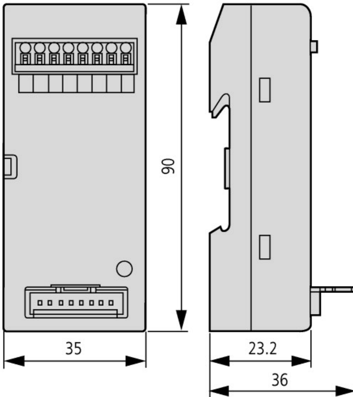
Component adapter flat cable (plug) on round cable (terminal) Adapter flat cable on round cable
