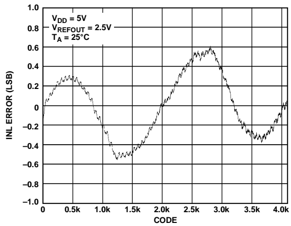
Figure 12. INL—AD5623R-5
