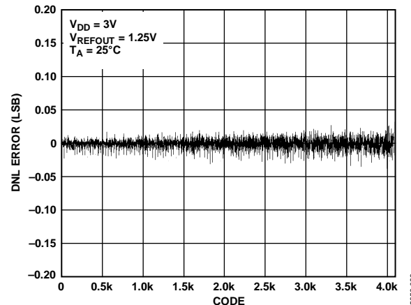
Figure 21. DNL—AD5623R-3
