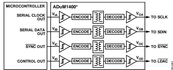
Figure 88. Isolated Interface
