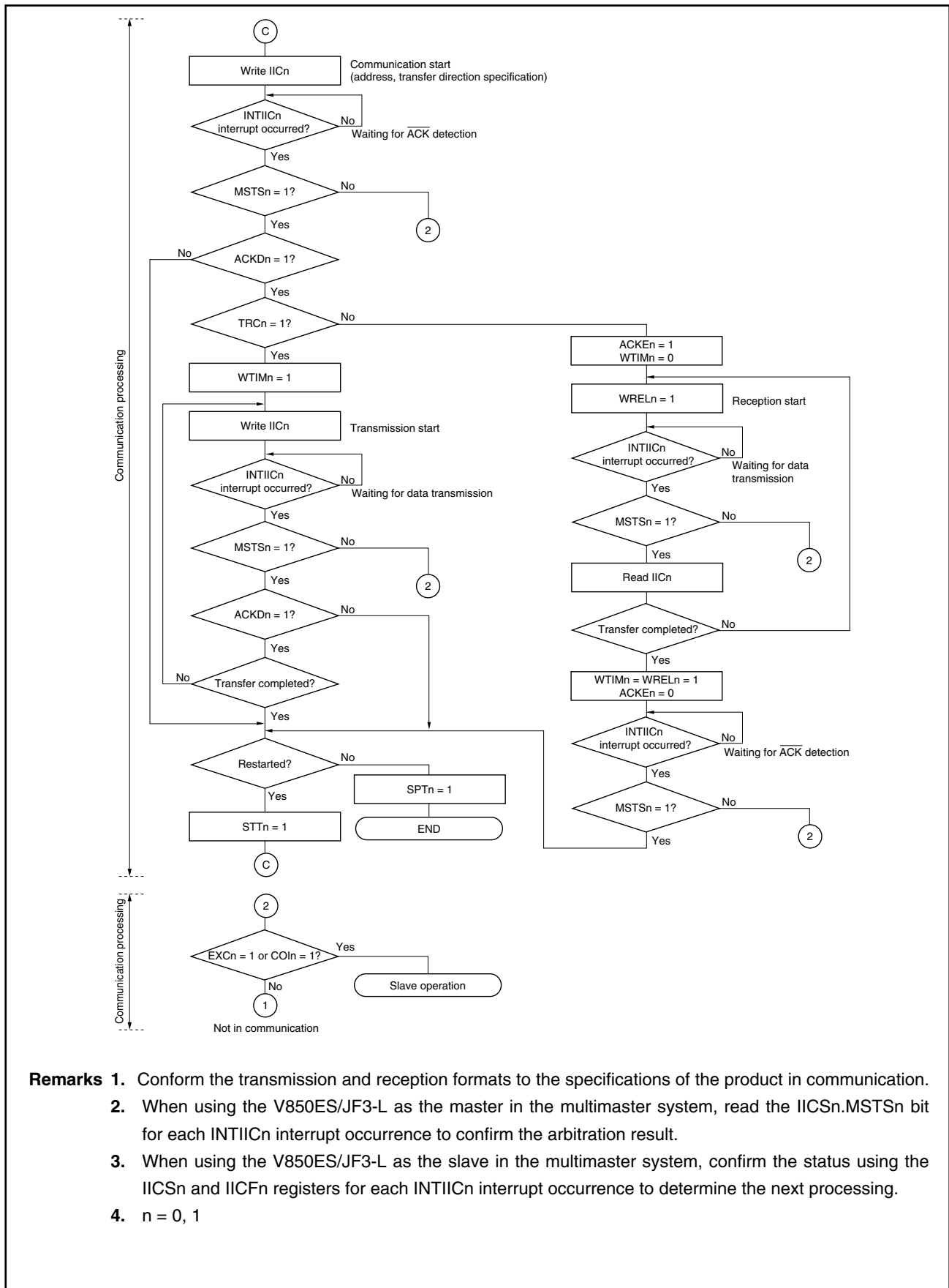
Figure 17-18. Master Operation in Multimaster System (3/3)
