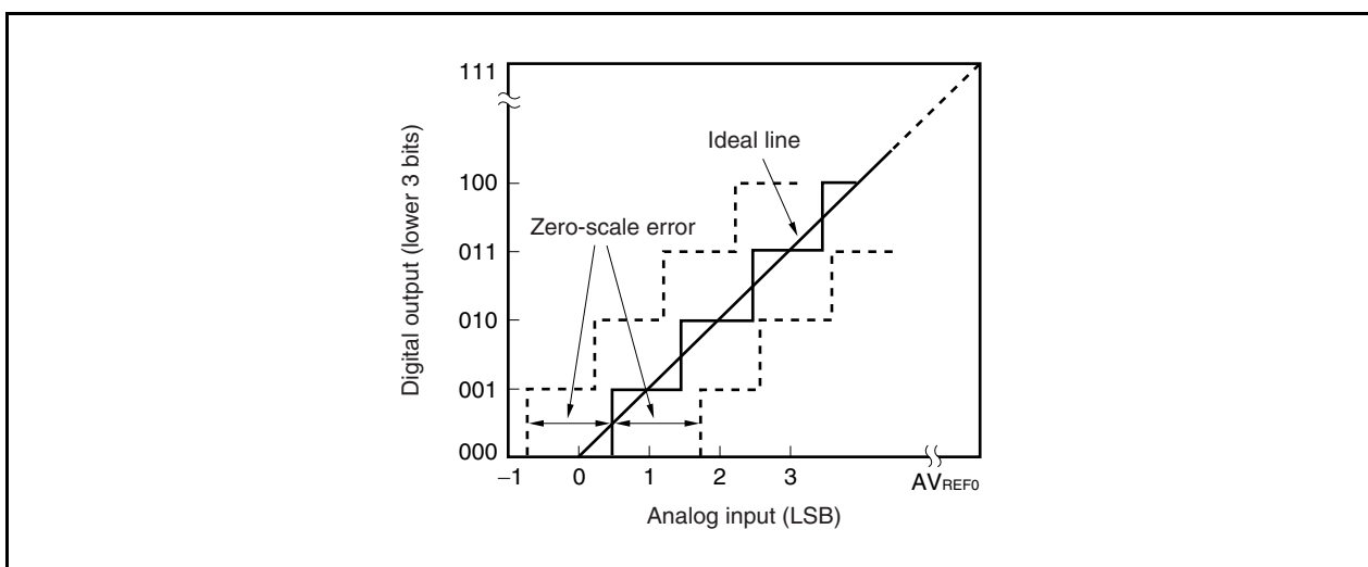
Figure 13-18. Zero-Scale Error
