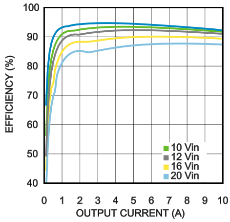
Efficiency, V_{OUT} = 5.0V
