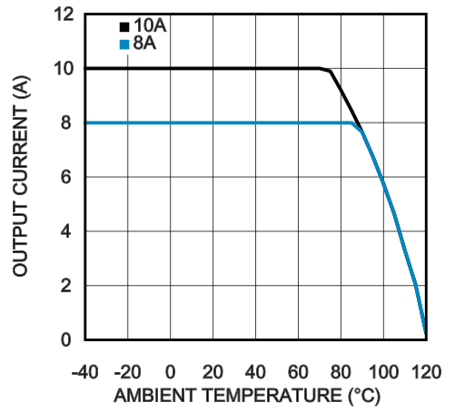
Thermal Derating, V_{OUT} = 5.0V
