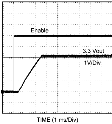
Startup, V_{IN} = 12V , V_{OUT} = 3.3V
