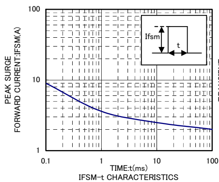
IFSM-t CHARACTERISTICS
