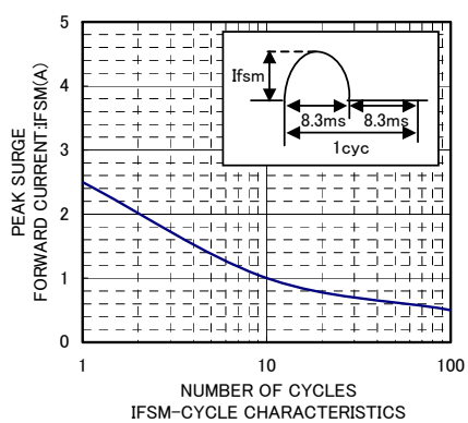
IFSM-CYCLE CHARACTERISTICS
