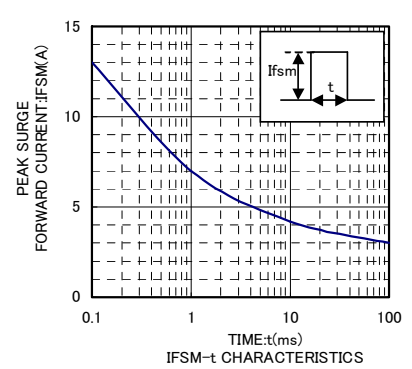
IFSM-t CHARACTERISTICS
