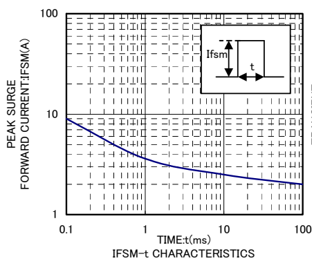
IFSM-t CHARACTERISTICS
