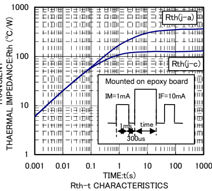
Rth-t CHARACTERISTICS
