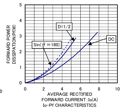
Io-Pf CHARACTERISTICS
