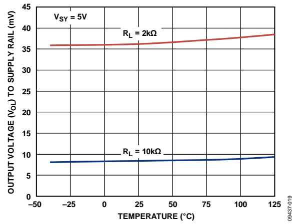
Figure 23. Output Voltage ( V_{OI} ) to Supply Rail vs. Temperature
