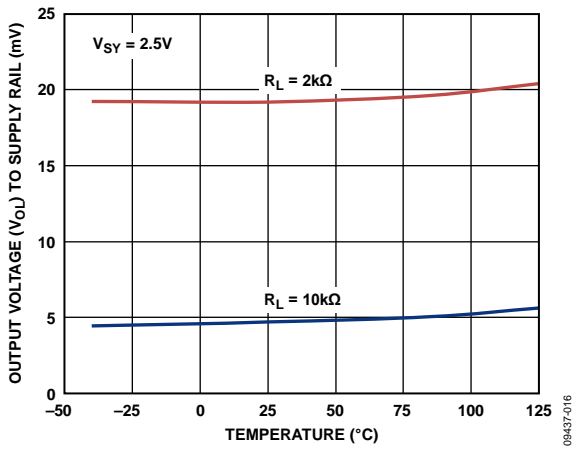
Figure 20. Output Voltage ( V_{OI} ) to Supply Rail vs. Temperature
