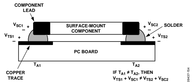
Figure 65. Mismatch in Seebeck Voltages Causes Seebeck Voltage Error
