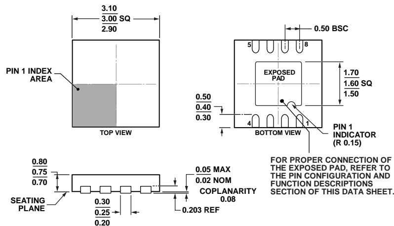
Figure 67. 8-Lead Lead Frame Chip Scale Package [LFCSF_WD] 3 mm x 3 mm Body, Very Very Thin, Dual Lead (CP-8-12)
