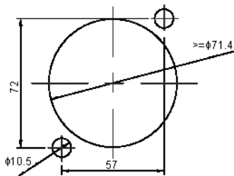
Panel Cut Out (rear side)
