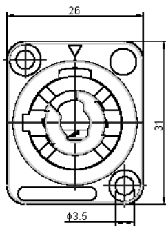
Panel Cut Out (rear side)
