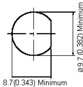
Mounting Hole Scale 3:1
