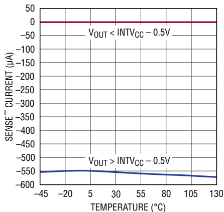
SENSE - Pin Total Input Current vs Temperature
