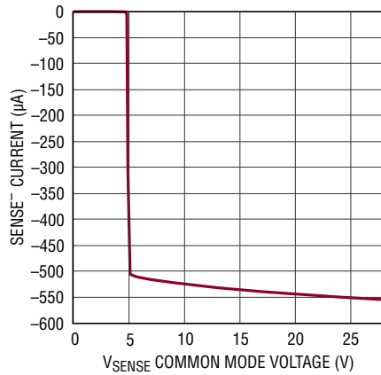
SENSE - Pin Total Input Bias Current
