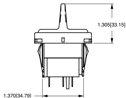
8 TERMINAL BASE W/O BARRIERS
