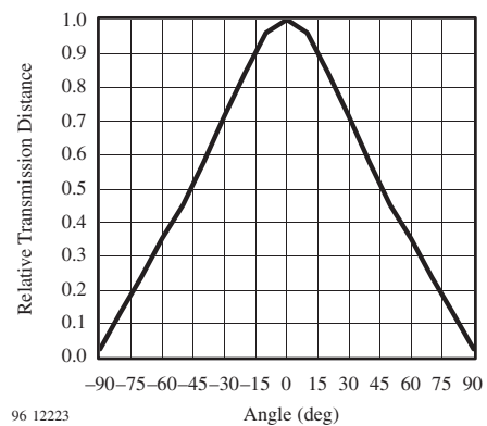
Figure 12. Directivity
