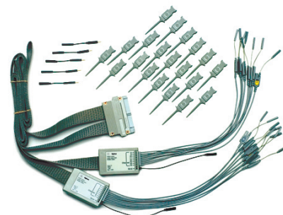
54620-68701 logic probe
