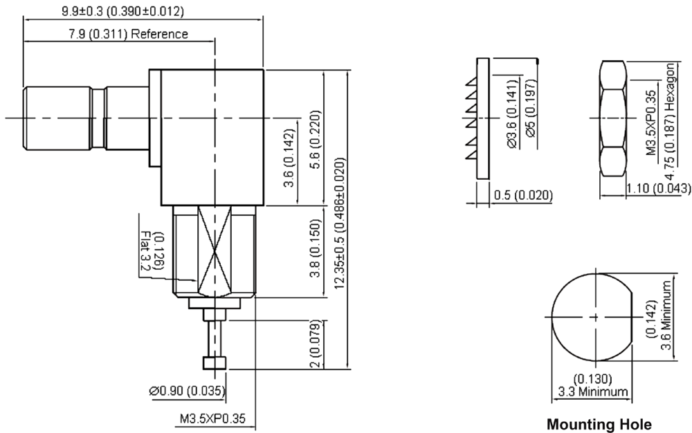
Mounting Hole
