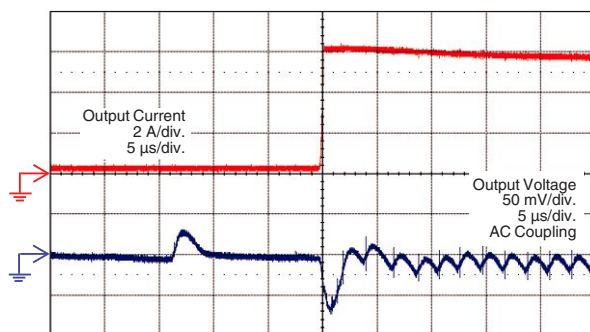
Transient Response in Power Save Mode (0.2\text{ A} - 6\text{ A}) (V_{IN} = 12\text{ V}, V_{OUT} = 1\text{ V}, F_{SW} = 500\text{ kHz at } 6\text{ A})
