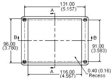
Assembly - Top
