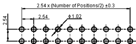
PCB Layout
