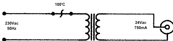
SCHEMATIC
