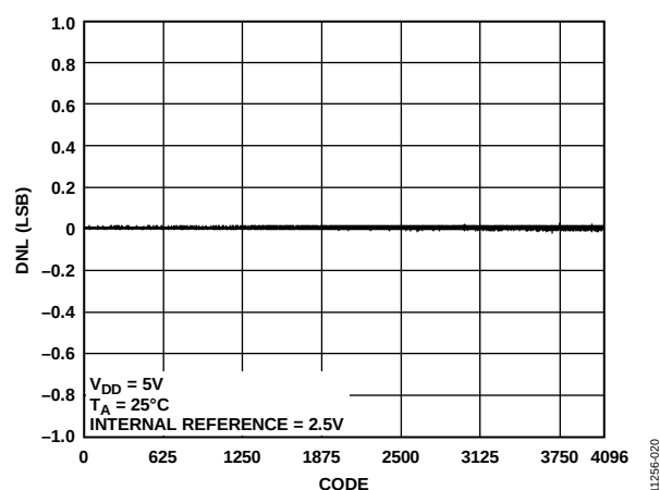
Figure 19. AD5687R DNL vs. Code
