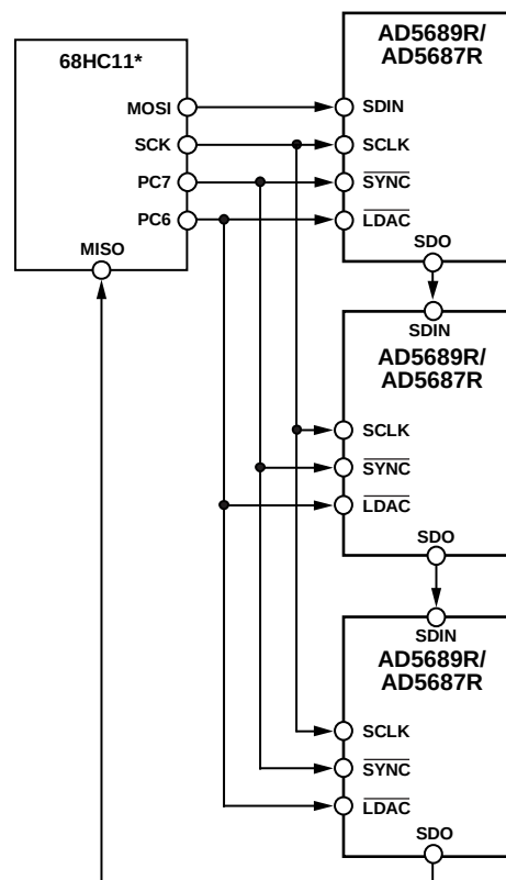
Figure 46. Daisy-Chaining Multiple AD5689R/AD5687R Devices
