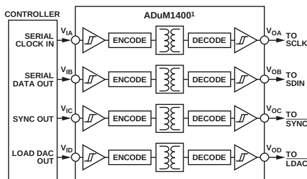
Figure 55. Isolated Interface
