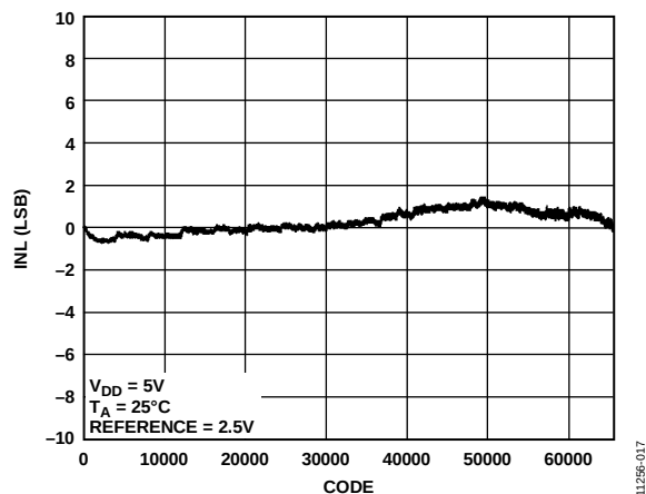
Figure 15. AD5689R Integral Nonlinearity (INL) vs. Code
