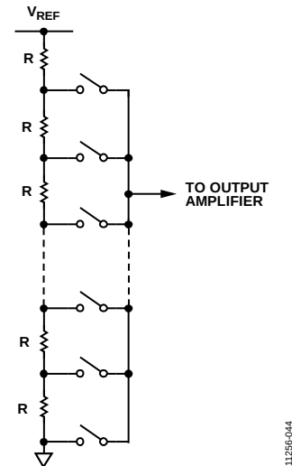
Figure 43. Resistor String Structure
