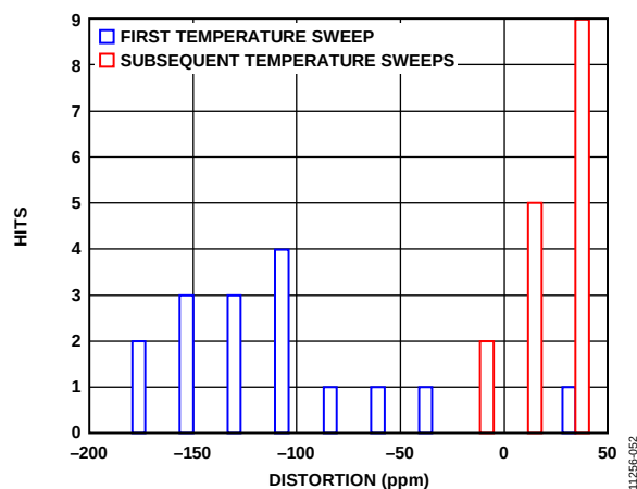
Figure 51. Thermal Hysteresis
