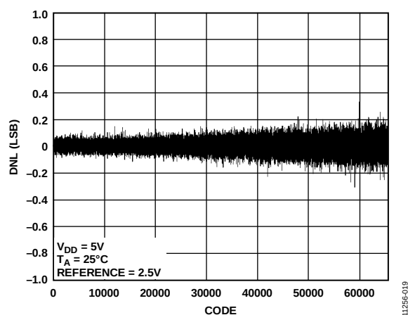
Figure 16. AD5689R Differential Nonlinearity (DNL) vs. Code
