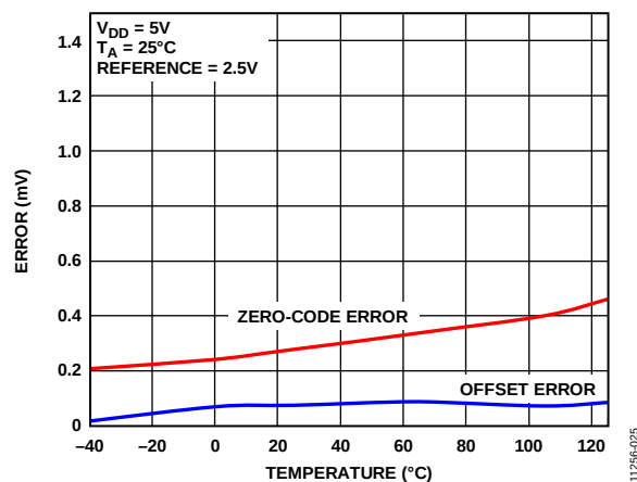
Figure 24. Zero-Code Error and Offset Error vs. Temperature
