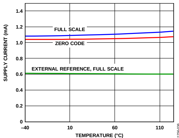
Figure 35. Supply Current vs. Temperature
