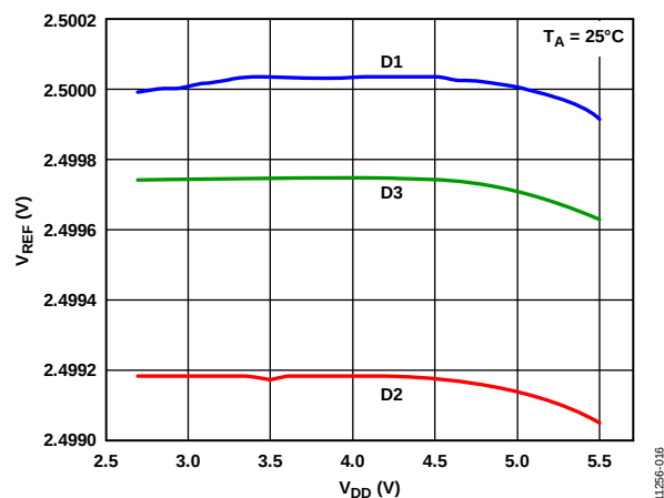
Figure 17. Internal Reference Voltage vs. Supply Voltage
