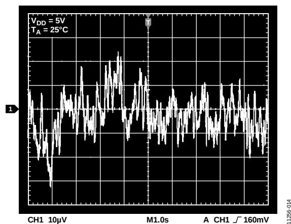
Figure 13. Internal Reference Noise, 0.1 Hz to 10 Hz
